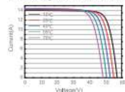
Current-Voltage Curve JAM78D40-610/GB
